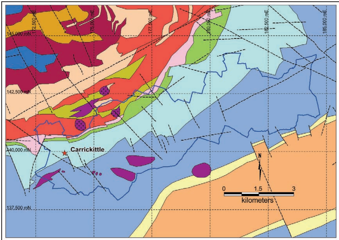
Figure 19: Carrickittle Block Geology and Mineral Occurrences
