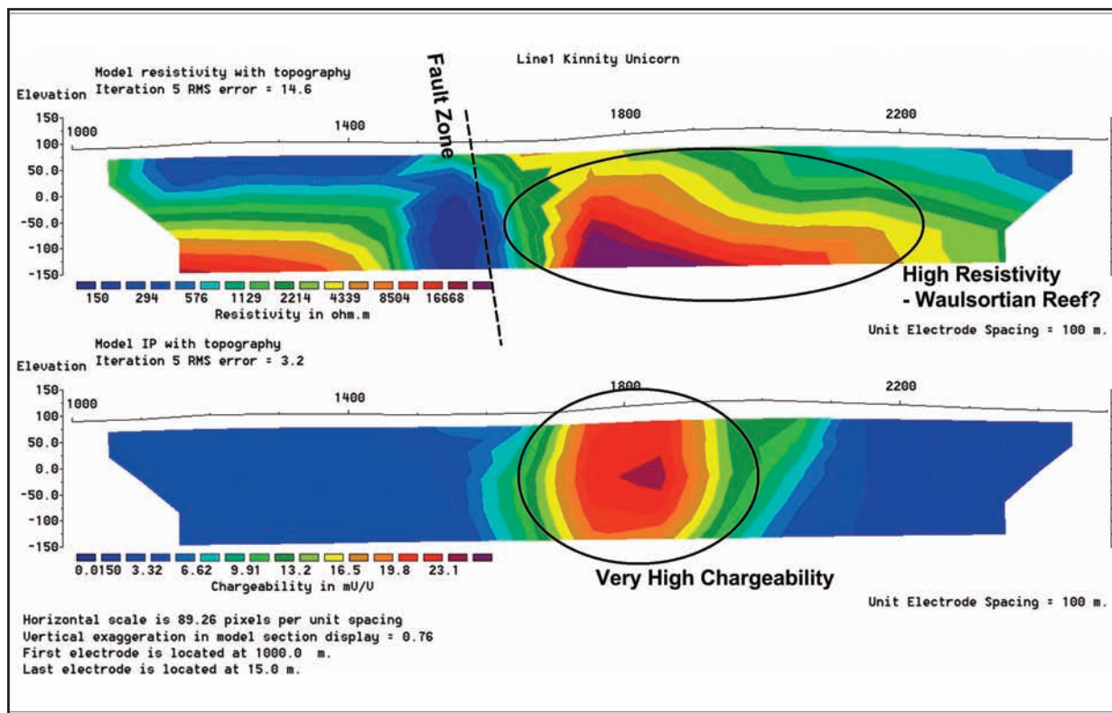
Figure 13: Kinnity IP Line 1, Inversion Pseudosection
