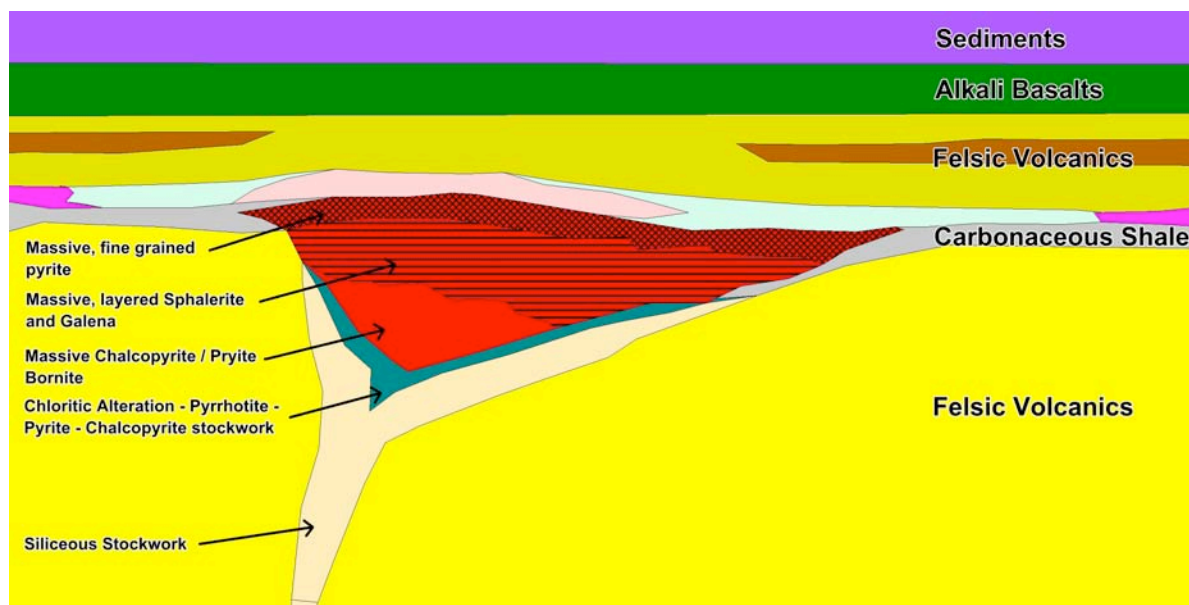
Figure 8: Schematic section through a VMS Zn/Pb/Cu deposit (model)
