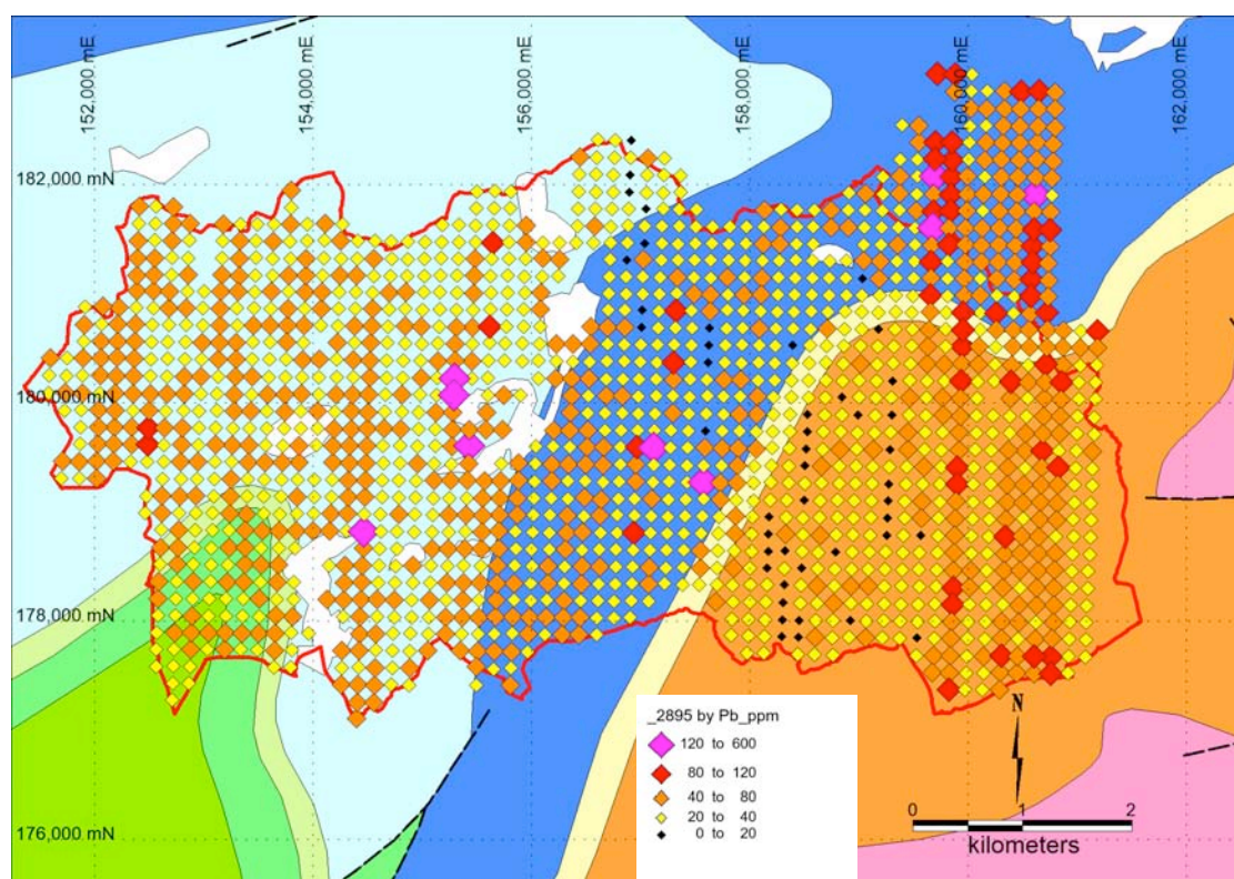
Figure 7: Pb Soil Geochemistry Poster-plot on Geology Background
