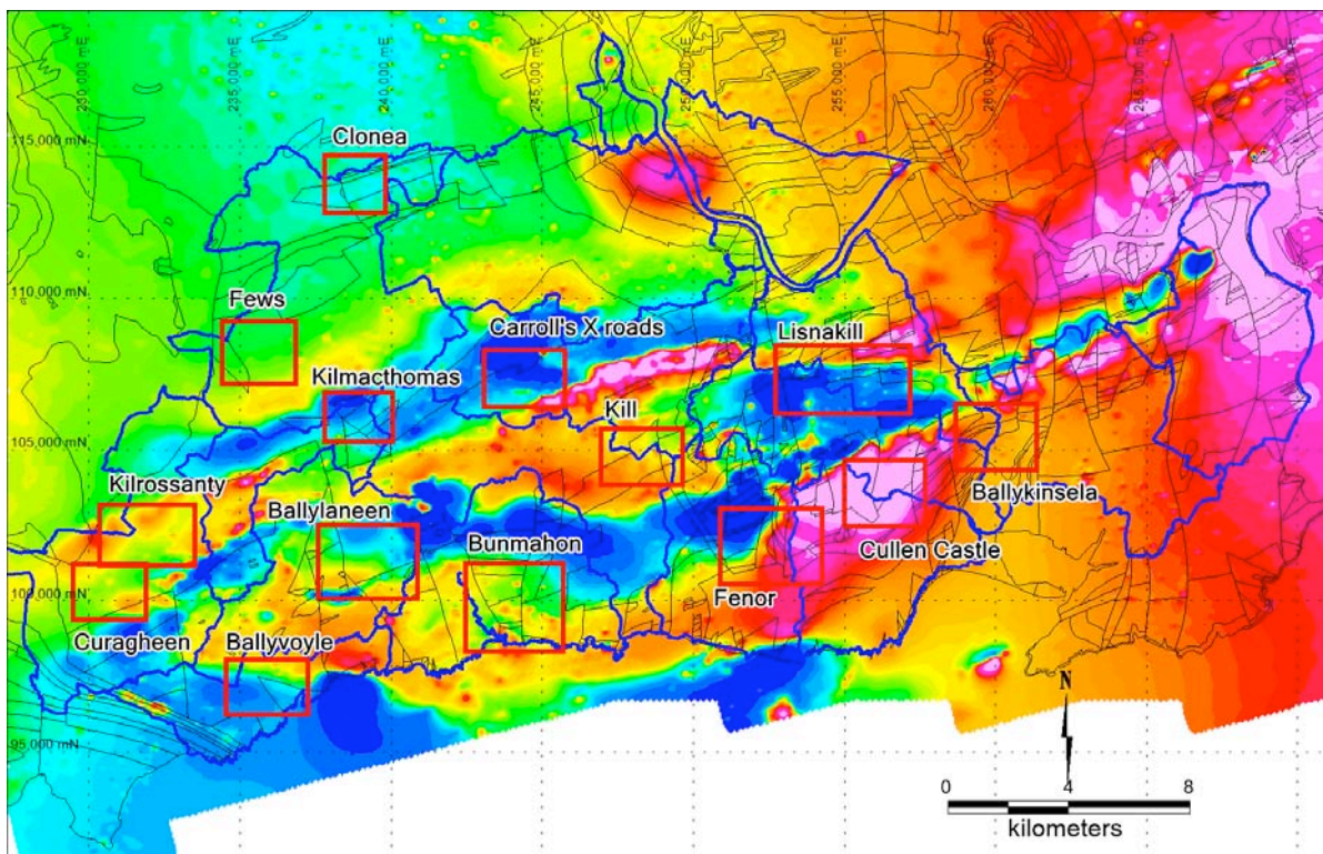
Figure 10: Waterford - airborne magnetic survey, target areas
