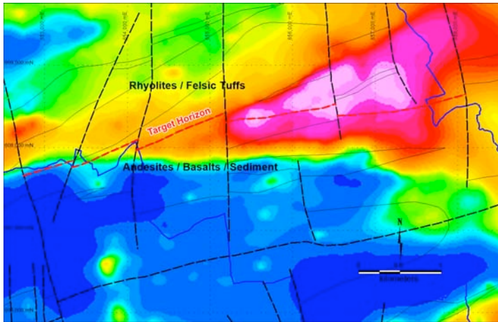
Figure 12: Lisnakill airborne magnetics - Note: displacement of contact to the south
