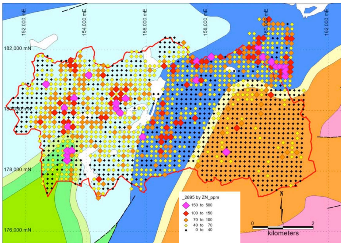
Figure 6: Zn Soil Geochemistry Poster-plot on Geology Background
