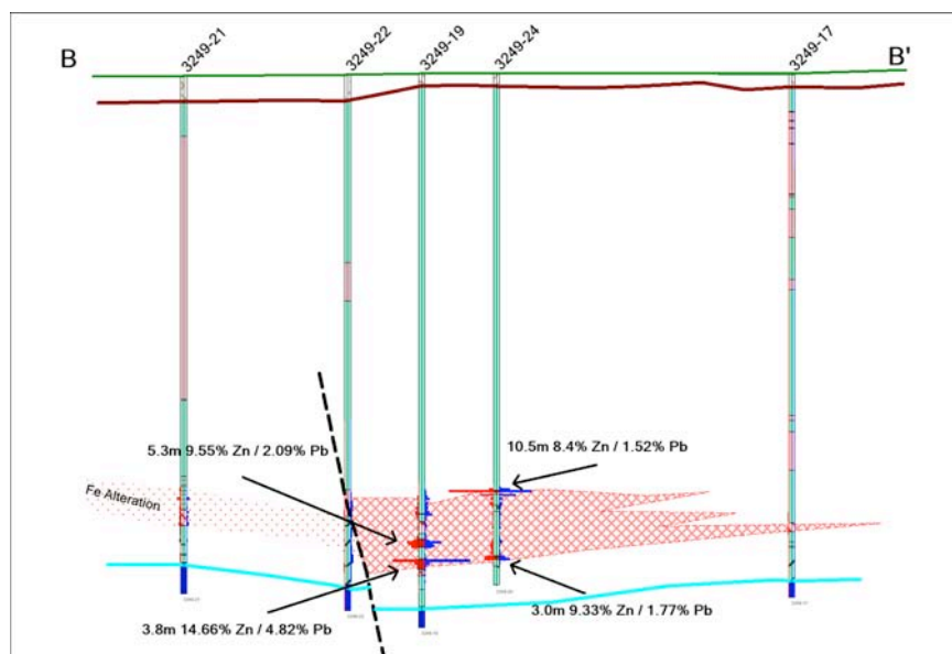
Figure 18: Cross section B - B'
