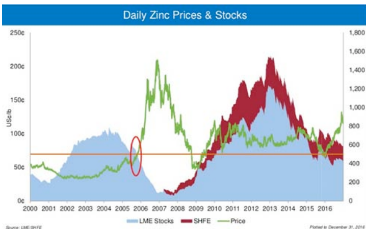
17 year zinc prices / stocks
