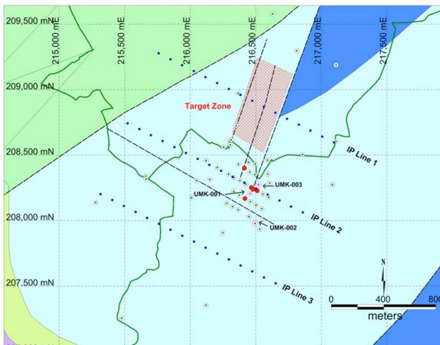
Figure 20: Drillhole collars at the Kinnity deposit, (including UMR drillholes UMK-001, 002 & 003)
