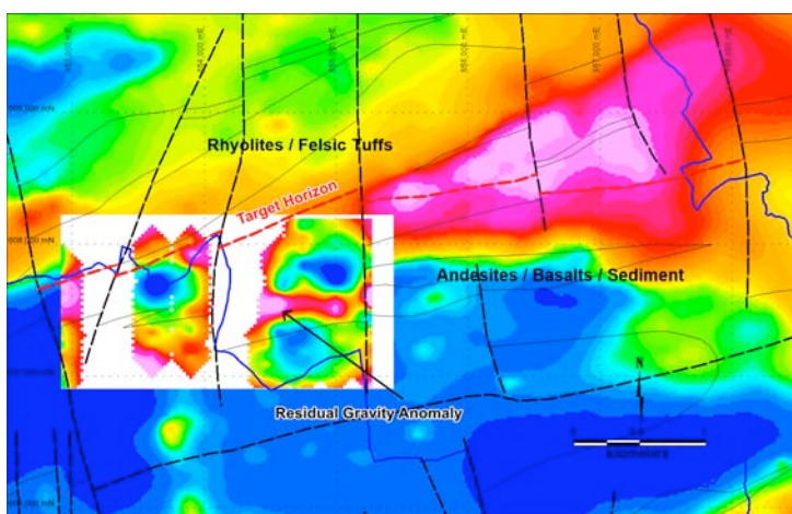
Figure 14: Lisnakill residual gravity, on magnetics and geology
