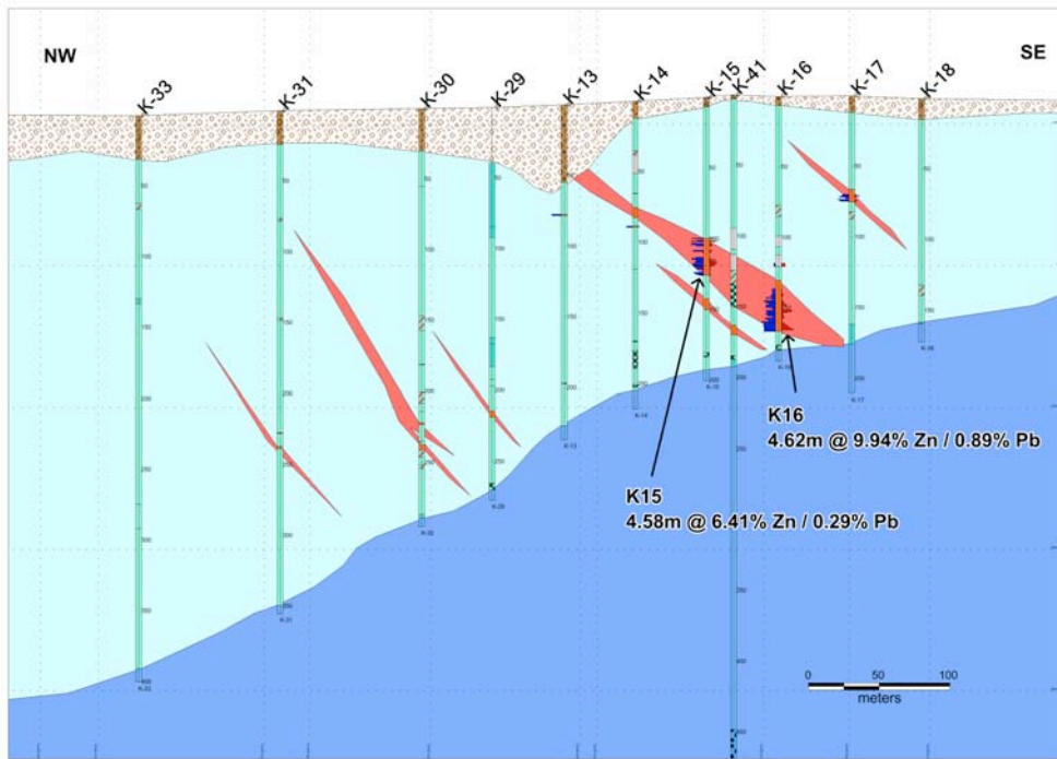
Figure 21: Drill section across the Kinnity deposit
