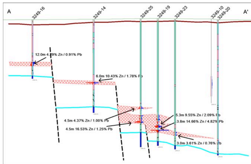
Figure 17: Cross section A - A'
