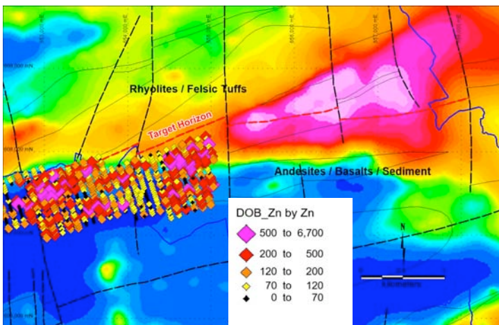
Figure 13: Lisnakill deep overburden sampling - zinc, on magnetics and geology
