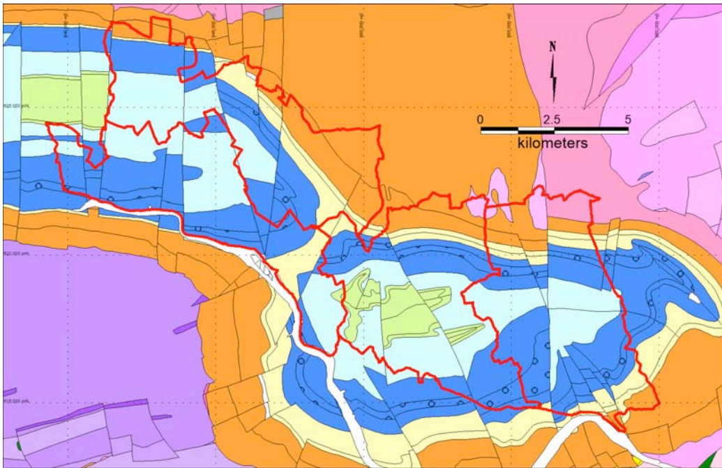
Figure 22: Clonmel geology map
